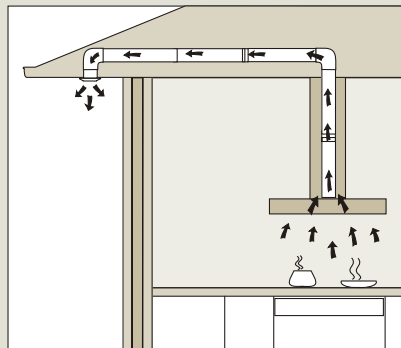
Side Exhaust to atmosphere
